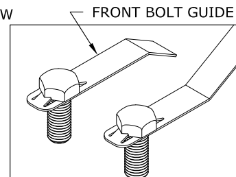
FIGURE C2: Bolt Guides REAR BOLT GUIDE
