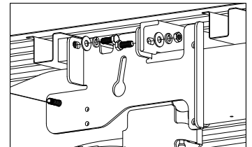
FIGURE C6: View from outside of Driver Side Frame.
